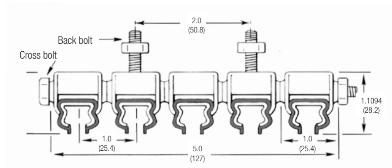
Standard Hangers
